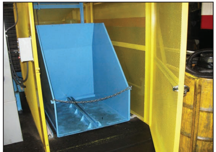
Cart Dumper with T-Rail Hold Down Feature
